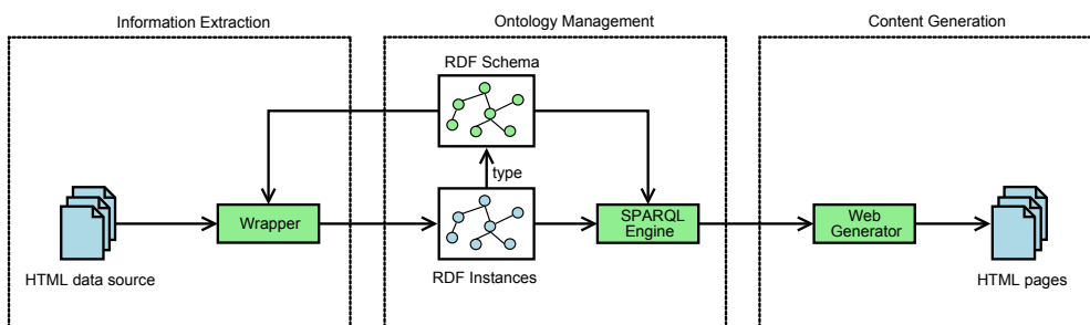
Figure 1. QMap information flow.
